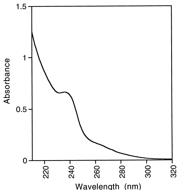
Figure 1. Absorption spectrum of 4'-(selenocyanato)phenylalanine 1 (0.0928 mM in 65% methanol).
