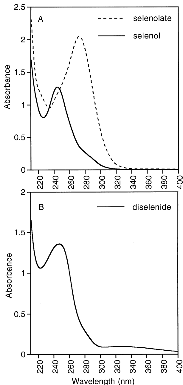
Figure 3. Absorption spectra of selenotyrosine 4 . A NaBH 4 (50 \mu L 0.5 M) was added to 0.123 mM 4'-(SeO 2 - )Phe in N 2 -sparged water (final volume 2 mL). The spectrum of the borohydride-generated selenotyrosine sample was recorded immediately (dashed line, selenolate) or after acidification to pH 2.2 with 40 \mu L 1 M HCl (solid line, selenol). B Spectrum of selenotyrosine diselenide 6 recorded 16 h after sample (a) was opened to air.
