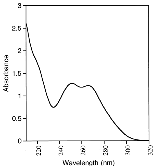
Figure 2. Absorption spectrum of 4'-(methylselenanyl)phenylalanine 2 . The crystalline compound was dissolved in 65% methanol and scanned against a solvent reference solution. The sample concentration was 0.167 mM, determined by Se analysis.
